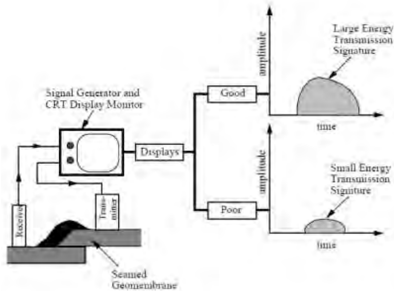
(c) Typical response signals
